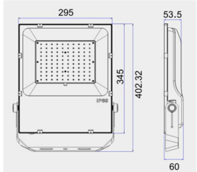
Dimension (mm)
